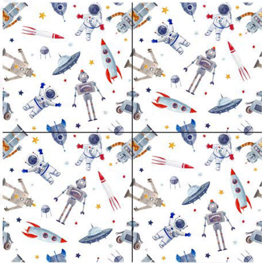
KC 09 (RANDOM)
